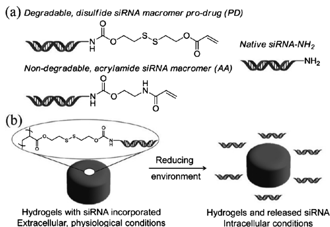
Figure 4. a) Structures of degradable and nondegradable siRNA macromers as well as native siRNA. b) Illustration of pro-siRNA hydrogel behavior under physiological and intracellular conditions. Adapted from Ref. [22]; copyright 2012 American Chemical Society.
