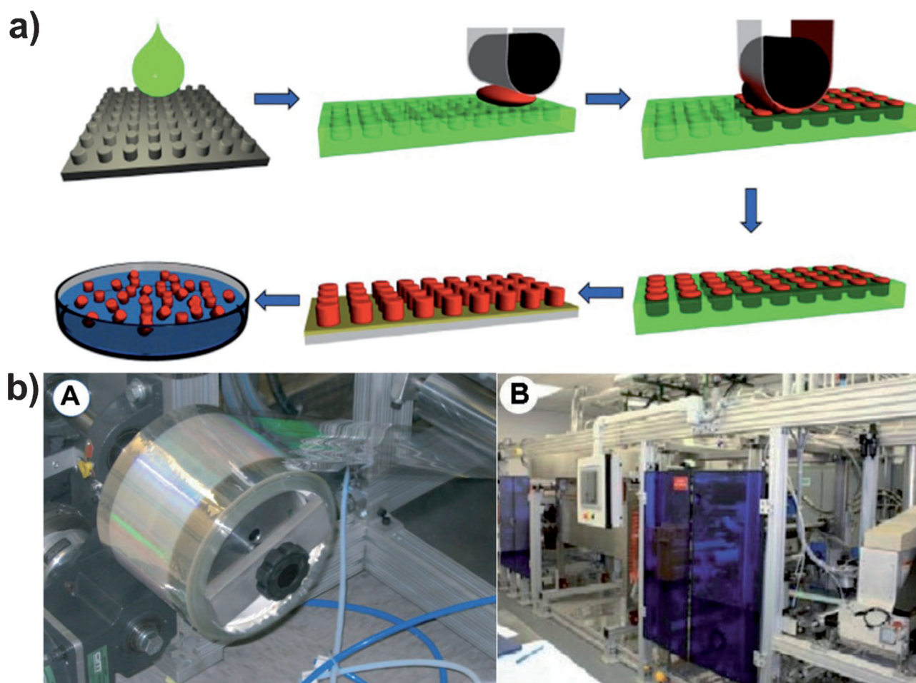
Figure 1. a) Preparation of PRINT mold and fabrication of PRINT particles. A liquid PFPE precursor can completely wet the silicon wafer with micro- and nanosized patterns because of its positive spreading coefficient on almost all surfaces and can be photocured to generate an elastomeric PRINT mold with negative micro/nanofeatures derived from the patterns on the silicon wafer. A liquid pre-particle material (red) is filled into the cavities without wetting the land area surrounding the cavities using a roll-to-roll process which involves a film-split technique against a high-surface-energy polyethylene terephthalate (PET) counter sheet when passed through a nip of a roller which applies pressure to the mold. The liquid in the mold cavities is then converted into a solid through a number of different processes including photocuring, or perhaps through vitrification by filling at an elevated temperature and cooling down, or by solvent evaporation. Once the liquid in the mold cavities is solidified, the array of particles (red) can be removed from the mold by bringing the mold in contact with an adhesive layer (yellow) which can pull the particles from the low-surface-energy mold. The particles can now be easily freed from the surface by dissolving the adhesive layer. b) Technical innovations in the PRINT technology: A) a roll of low-cost thin mold for PRINT particle fabrication and B) a roll-to-roll equipment for continuous PRINT particle manufacturing. Adapted from Ref. [14] with permission from Future Medicine Ltd.
